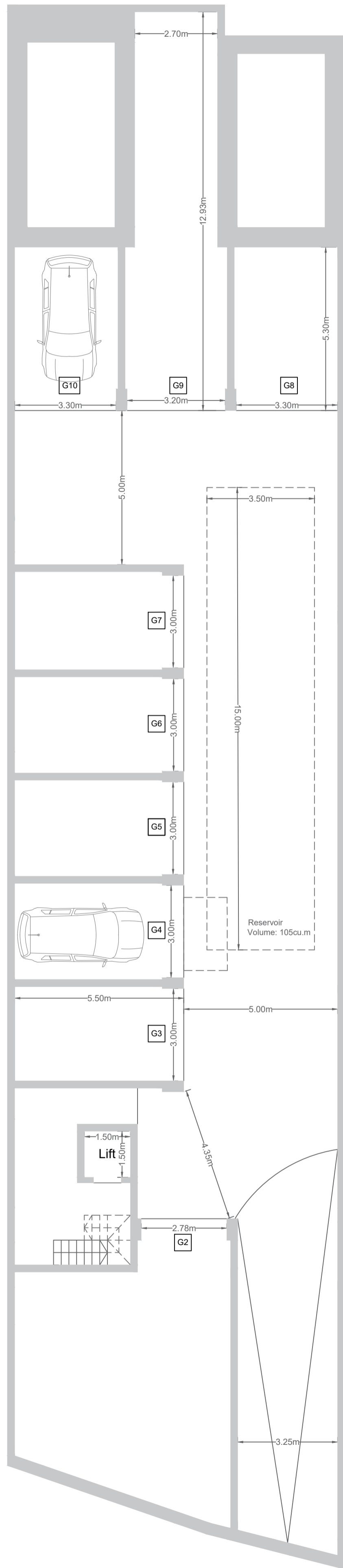
PROPOSED BASEMENT LEVEL SCALE 1:100
