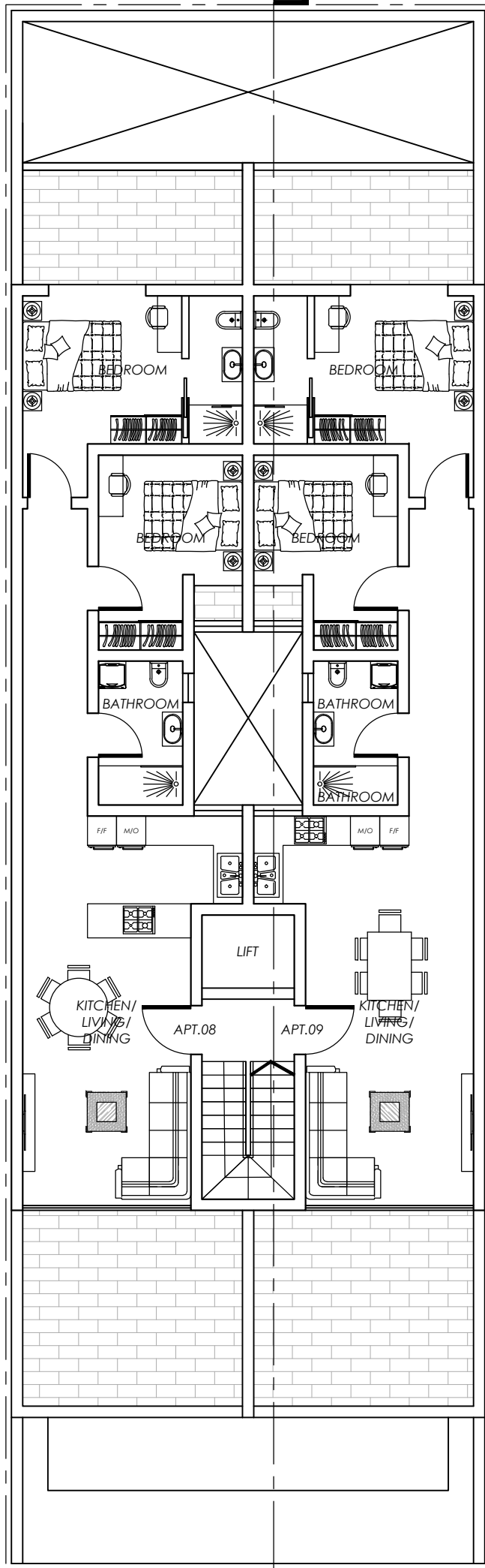
DRAWING | RECEDED FLOOR LEVEL SCALE | 1:100
